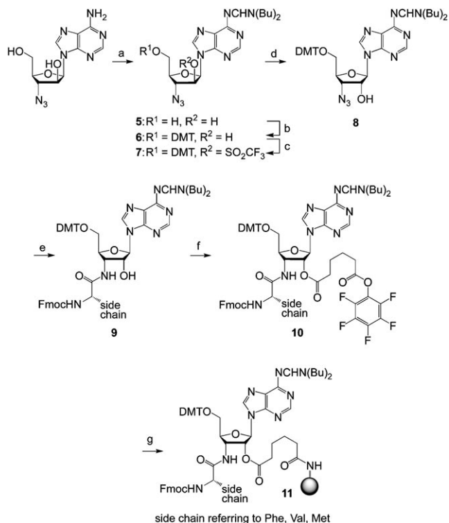
Scheme 2. Synthesis of the 3'-amino-3'-deoxyadenosine-functionalized support 11 (rA 3'-NH ) for the automated solid-phase synthesis of RNA–peptide conjugates. Reagents and conditions: a) 4 equiv N,N -di- n -butylformamide dimethyl acetal, DMF, 80 °C, 2.5 h, 89%; b) 2 equiv DMT-Cl, 0.3 equiv Bu 4 NNO 3 , pyridine, RT, 1.5 h, 79%; c) 1.5 equiv trifluoromethanesulfonyl chloride, 1.5 equiv DMAP, 2.5 equiv ( i Pr) 2 NEt, CH 2 Cl 2 , 0 °C, then 30 °C, 15 min; d) 5.5 equiv CF 3 COO - K + , 1.5 equiv ( i Pr) 2 NEt, 2 equiv [18]crown-6, toluene, 80 °C, 2.5 h (68% over (c) and (d)); e) 1.3 equiv Fmoc-Val-OBt (alternatively, Phe or Met), 2.2 equiv P(CH 3 ) 3 , THF, 0 ° to RT, 16 h, 89%; f) 5 equiv PfpOOC(CH 2 ) 4 COOPfp, 1 equiv DMAP, DMF/pyridine (1:1), RT, 1 h, 71%; g) 3 equiv (w/w) amino-functionalized support (GE Healthcare, Custom Primer Support 200 Amino), 2 equiv pyridine, DMF, RT, 22 h, loading: 46 μmol g -1 . DMT = 4,4'-dimethoxytrityl, DMAP = 4-(dimethylamino)pyridine, Fmoc = N -(9-fluorenyl)methyloxycarbonyl.
